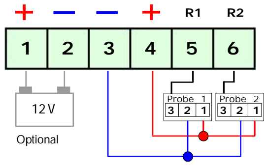
Connection of probes and eventual battery
