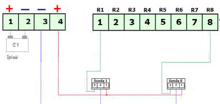
Connection of probes and eventual battery
